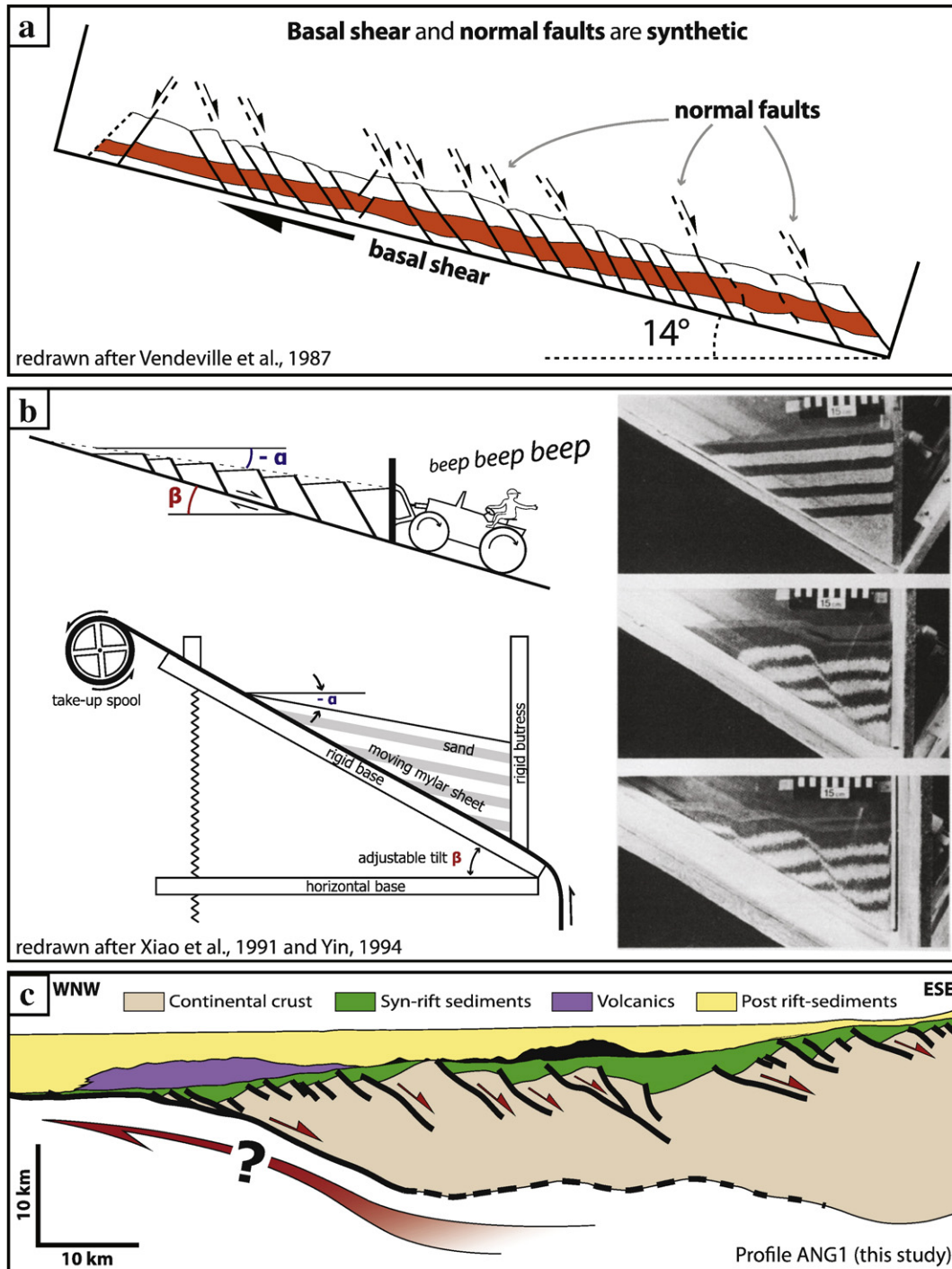
Fig. 15. a) Sand model uniformly stretched by downslope planar normal faults, redrawn after Vendeville, 1987. b) Sandbox experiment showing the progression of deformation sequence through an extensional wedge, photograph and redrawn from Xiao et al., 1991 and Yin, 1994. The locus of active synthetic normal faulting moves from the back to the front of the wedge (from right to left on the photograph). Comparison with profile ANG1 (c) suggests the existence a major shear at the base of the continental crust.
