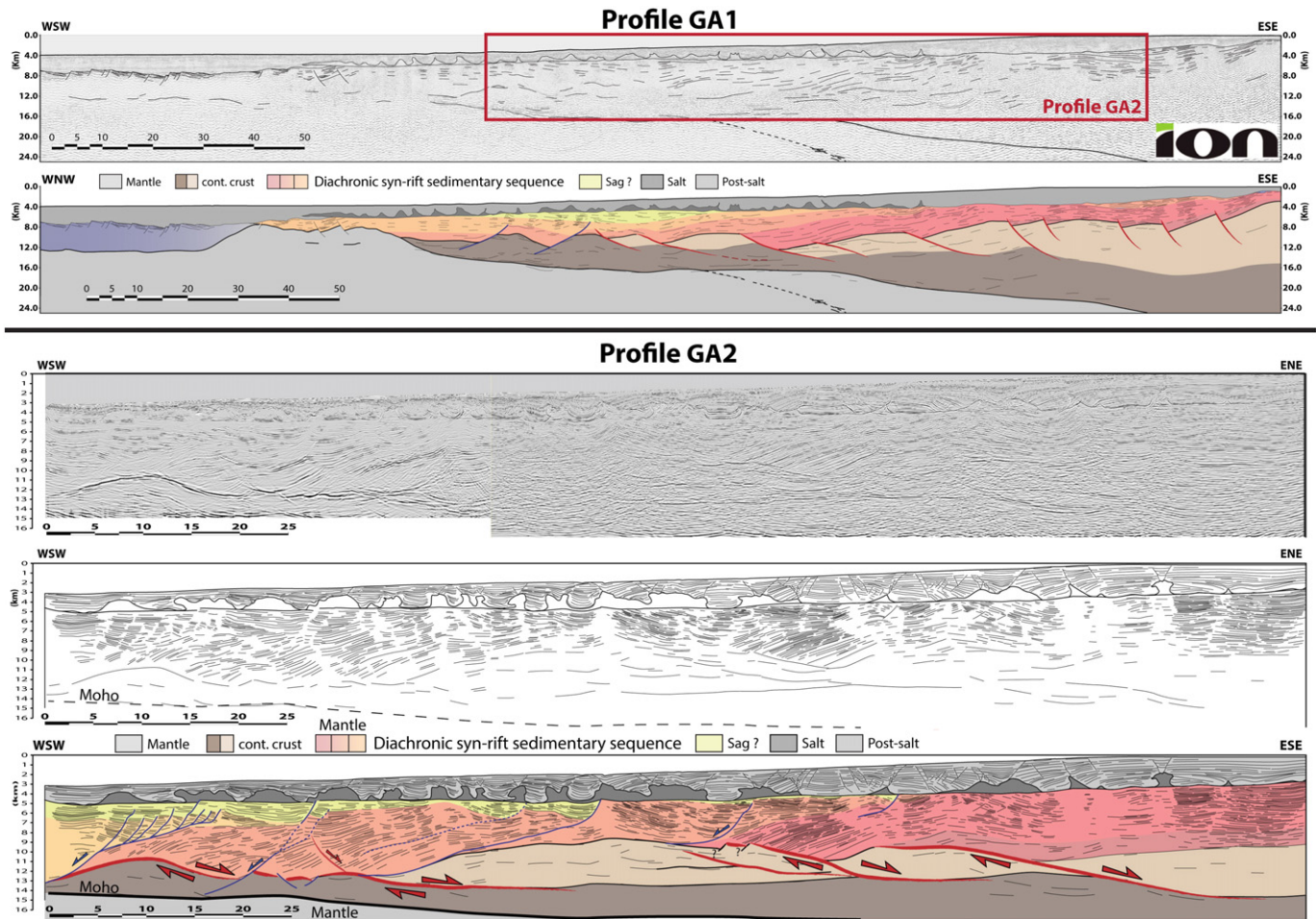
Fig. 7. Profiles 1 and 2 from the Gabon rifted margin. Both profiles are parallel and roughly superposed. Approximate projection of profile GA2 on profile GA1 in indicated by the red box. See map on Fig. 6 for location.
