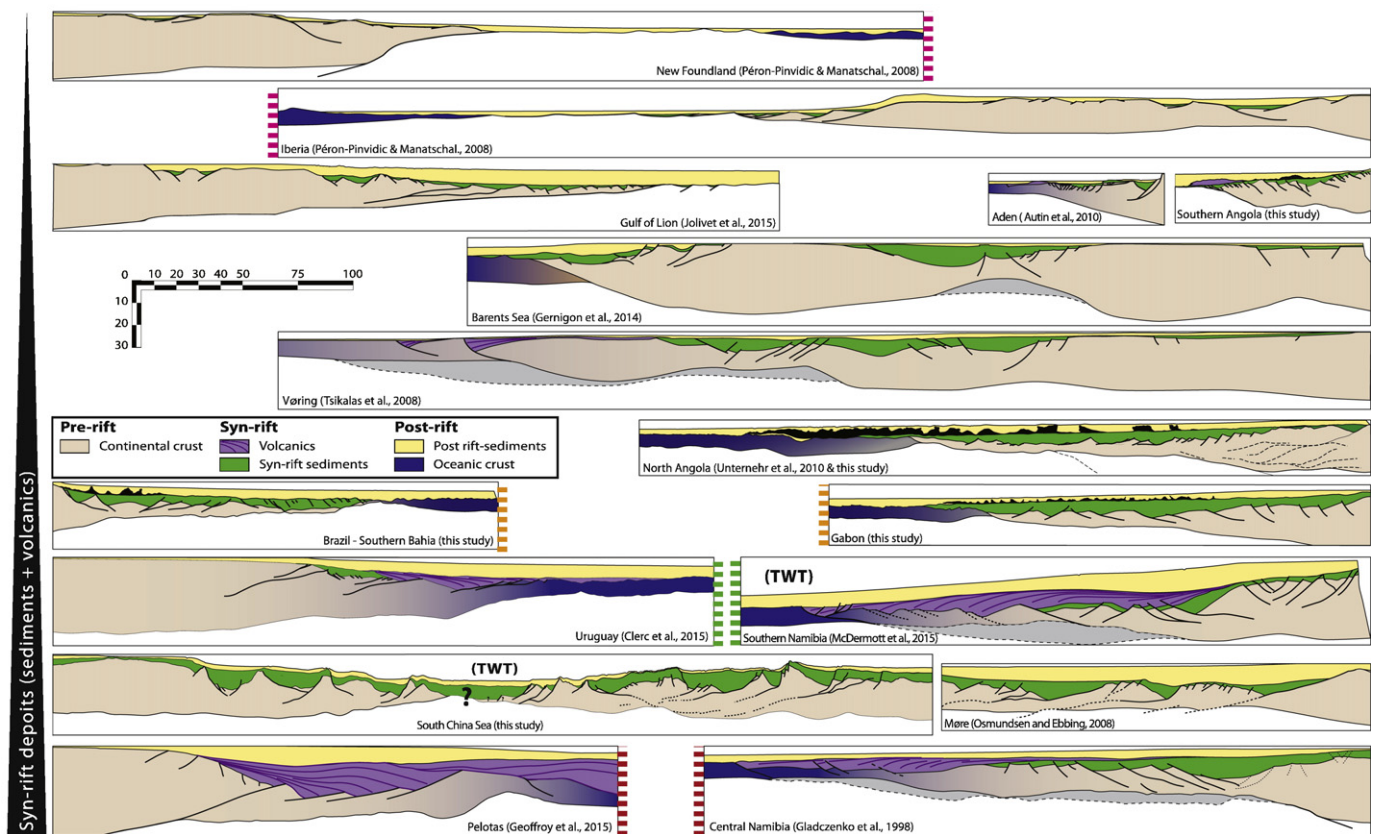
Fig. 2. Variability in length of the margin, abundance of syn-rift deposits (sediments and/or volcanics), dip direction of the normal faults and general crustal behavior of the continental crust at rifted margins. Compilation from 15 rifted margins from this study and reproduced from Péron-Pinvidic and Manatschal (2008), Autin et al. (2010), Jolivet et al. (2015), Gernigon et al. (2014), Tsikalas et al. (2008), Untermeier et al. (2010), Osmundsen and Ebbing (2008), Clerc et al. (2015a), McDermott et al. (2015), Geoffroy et al. (2015), Gladczenko et al. (1998).
