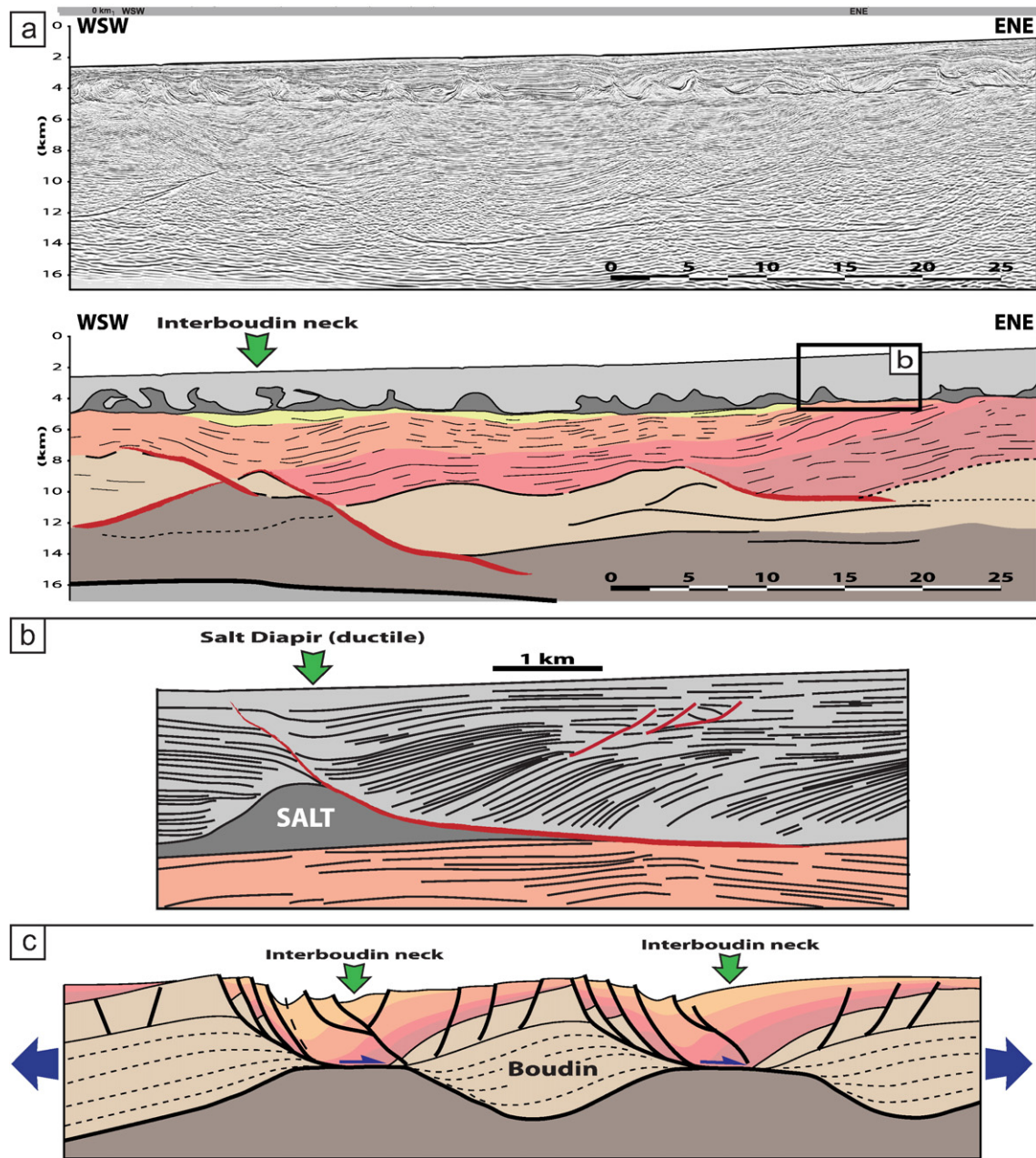
Fig. 14. a) interpretations of seismic profiles across the magma-poor margin of Gabon, a few tens of kilometers south of profile GA2. Courtesy of Total, Marathon and Cobalt. b) Comparison with similar structures observed at a completely different scale, in the rafted post-salt sediments. Localisation in (a). c) Comparison with a model of crustal boudinage, redrawn after Gartrell (1997).
