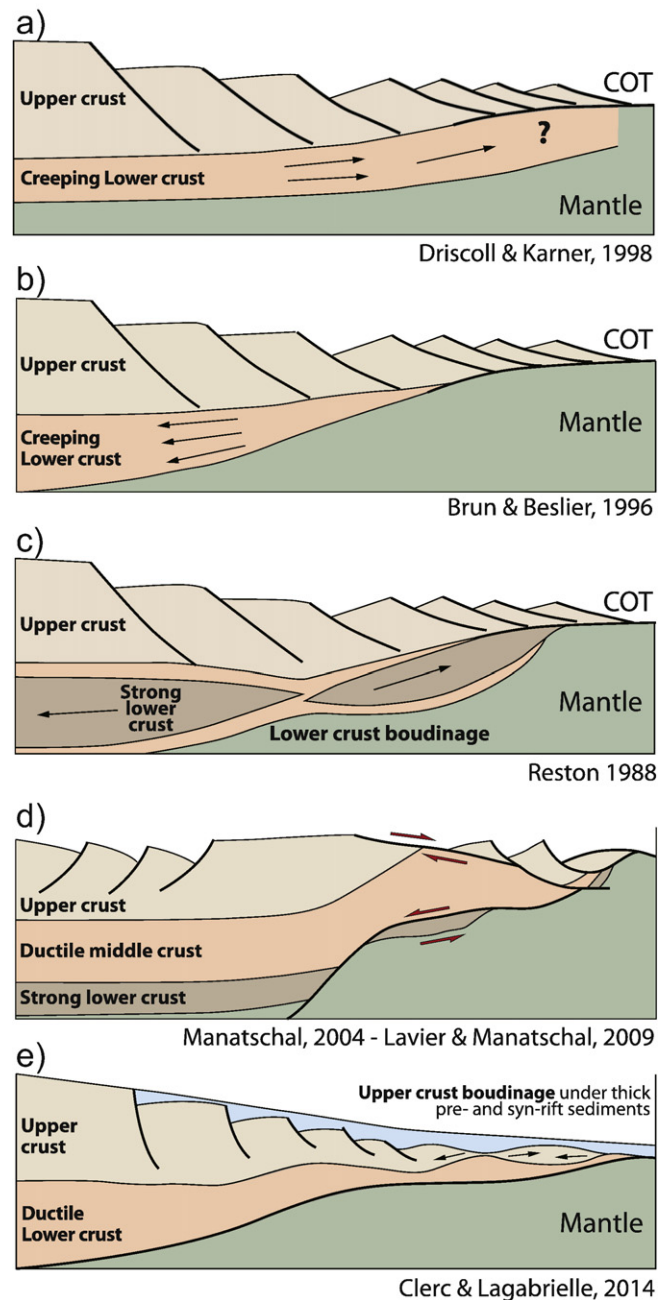
Fig. 1. Some of the many models proposed for the behavior of the continental crust during the formation of rifted margins. (Source: modified after Reston, 2007).
