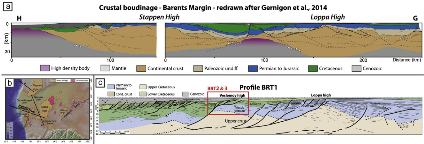
Fig. 12. a) Interpretation of the Barents margin redrawn after Gernigon et al. (2014). b) Localization map for profiles G, H, BRT1, BRT2 and BRT3, redrawn after Faleide et al. (1984) and Gernigon et al. (2014). c) Profile BRT1 across the Loppa and Veslemøy highs.
