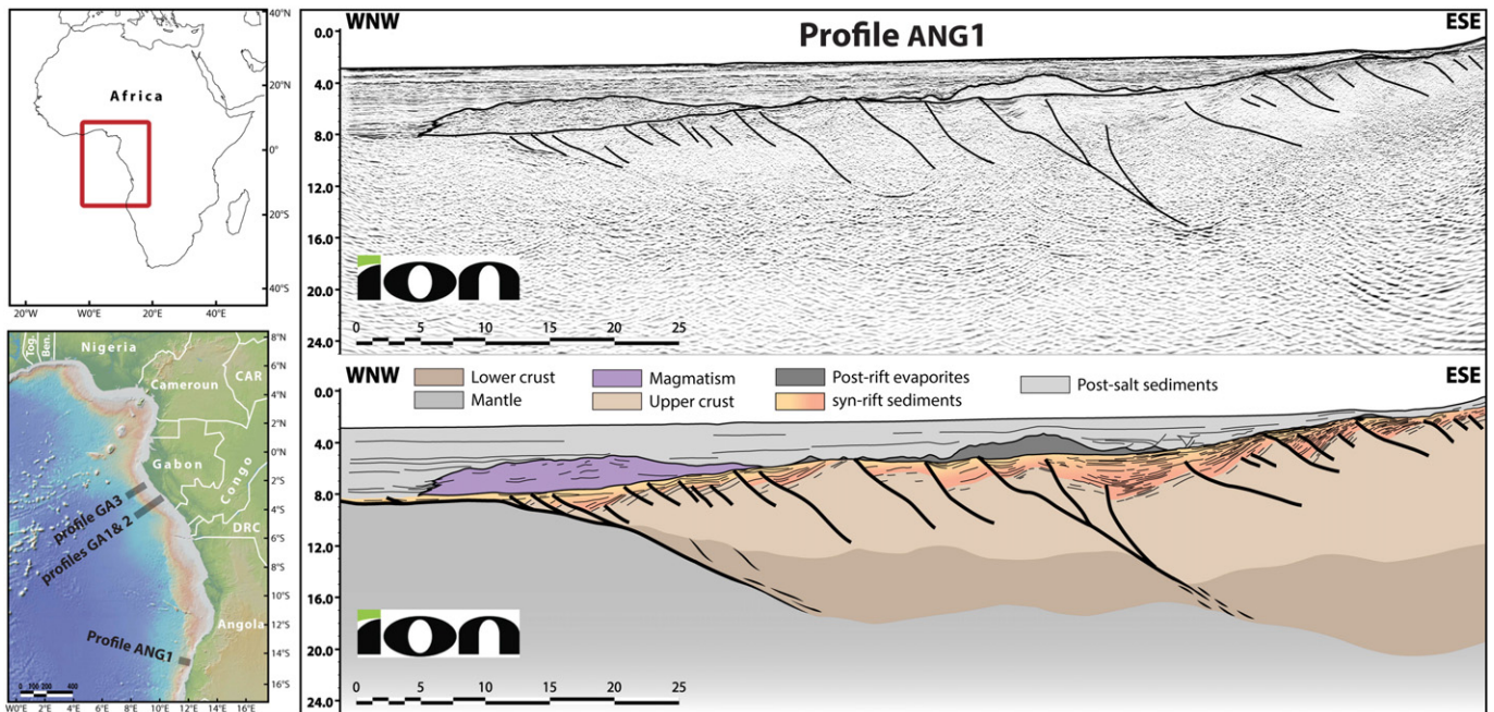
Fig. 6. Map of West Africa showing the localisation of profiles GA1, GA2, GA3 and ANG1. Basemap from http://www.geomapp.org and Ryan et al. (2009). Profile ANG1 and interpretation.
