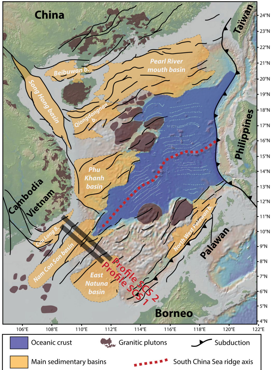
Fig. 9. Map of the South China Sea showing the main structural features, after Savva et al., 2013, 2014; Franke et al., 2014. Profiles SCS1 and SCS2 are located at the southwestern tip of the South China Sea propagator.
