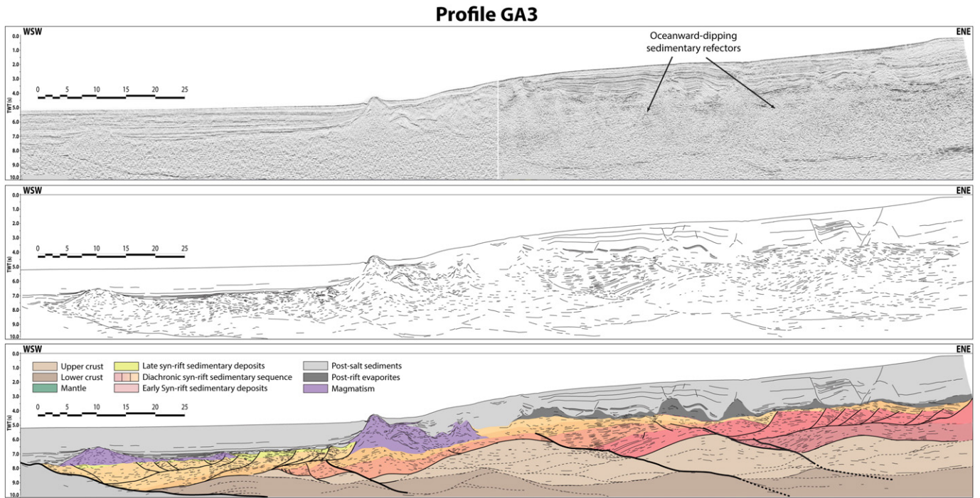
Fig. 8. Seismic reflection profile GA3, line-drawing and interpretation across the Gabon margin, >100 km north of profiles GA1 & GA2. See map on Fig. 6 for location. Source: Data courtesy of Schlumberger Multiclient and Petrolin.
