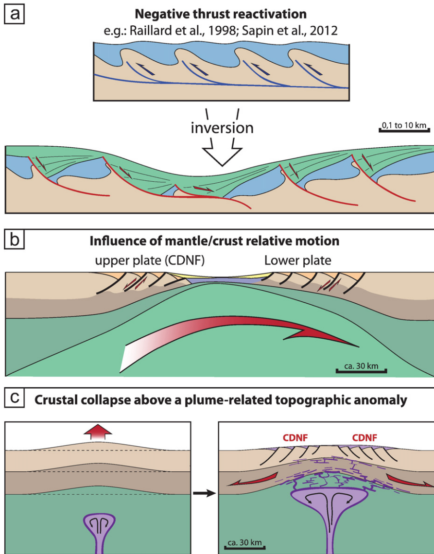
Fig. 16. Possible scenario for the formation of Continentward Dipping Normal Faults (CNDF). a) Formation of CNDF by inversion of inherited structures (former thrusts), modified after Raillard et al. (1998) and Sapin et al. (2012); the formation of CNDF can also be controlled by the existence of top-to-the-continent shear at the base of the crust. This shear could result either from (b) a basal drag of the mantle due to mantle drift; or (c) in the case of volcanic rifted margins to the collapse of a topographic anomaly above an emerging plume.
