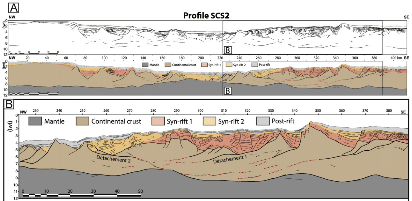
Fig. 11. A: Profile SCS2 across the Nam Con Son Basin, located 60 km northeast of profile SCS1. The seismic profile is available from Fig. 5A of Franke et al., 2014. B. Zoom on a crustal dome at the intersection of two antithetic detachments. Source: Data courtesy of TGS.
