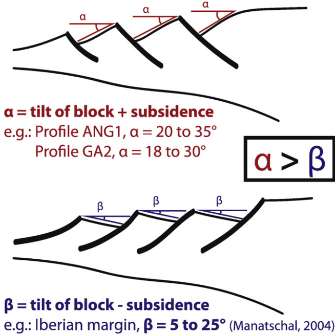
Fig. 17. Implication of fault dip on the tilt of the crustal blocks. On CDNF-controlled margins, bloc-related tilting adds up to the subsidence-related tilting. Whereas on margins controlled by oceanward-dipping normal faults, block tilting (toward the continent) is opposed to subsidence-related tilting (toward the ocean).
