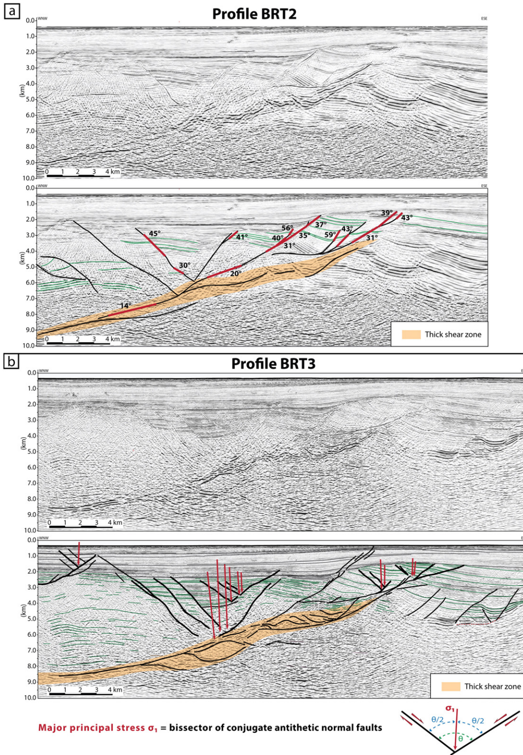
Fig. 13. Profiles BRT2 (a) and BRT3 (b) across the Veslemøy crustal high (data courtesy of Schlumberger). Nucleation of low angle normal faults is attested from profile BRT2 (a), which is orthogonal to the faults strike (determined from 3D seismic block). b) The major principal stress \sigma_1 is found vertical on BRT3 by determining the bisector of the conjugate antithetic normal faults, which attests for the absence of post-fault tilting. The low angle between the faults and the sedimentary bedding, and the tiny rotation of these series also confirms that the faults nucleate at low angle.
