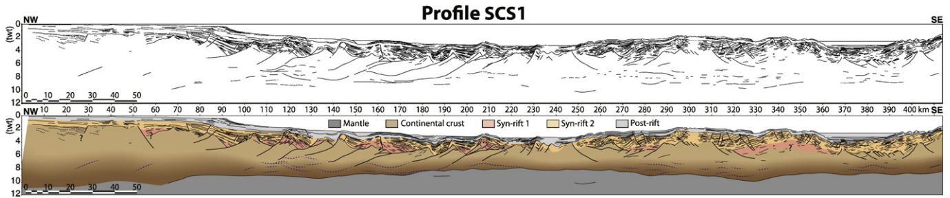
Fig. 10. Profile SCS1, across the Nam Con Son basin, located ahead the propagator of the South China Sea. Source: Data courtesy of TGS.
