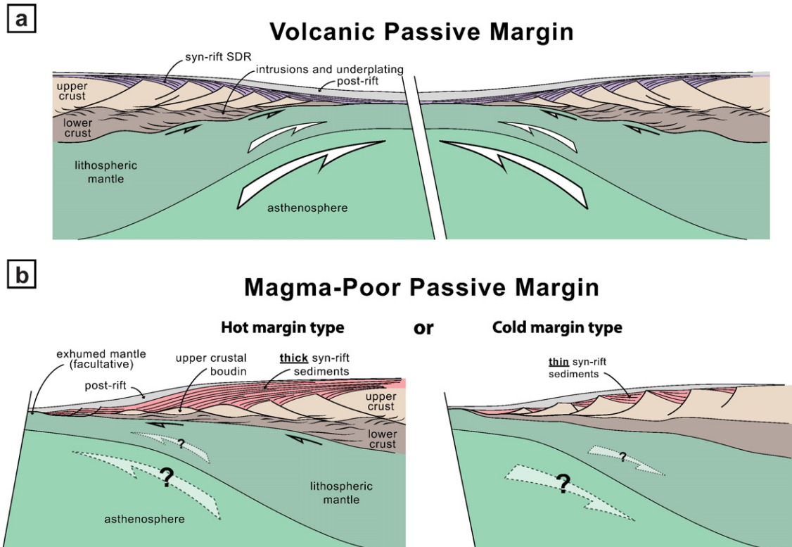
Fig. 18. Schematic representation of the volcanic rifted margins and ductile-type magma-poor rifted margin.
