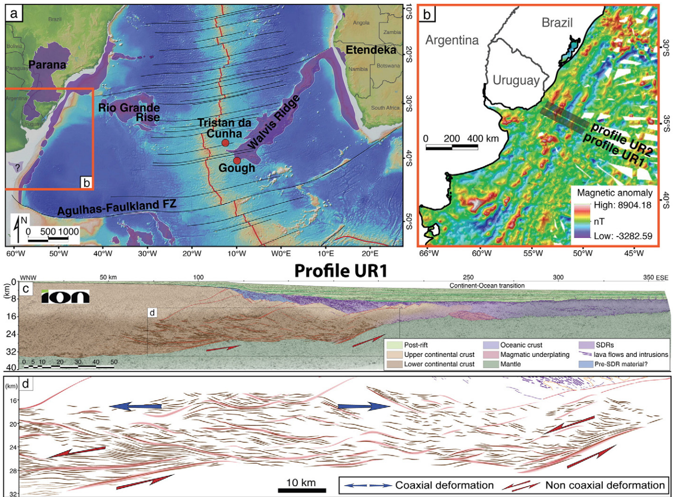
Fig. 4. a) Regional map of the southern Atlantic Ocean after Gladczenko et al. (1997), Stica et al. (2014) and Soto et al. (2011), basemap from http://www.geomapp.org and Ryan et al. (2009). b) Magnetic anomaly map of the Uruguayan rifted margin after Maus et al. (2009). c) Interpretation of profile UR1 and d) close-up on the shear patterns at the base of the lower crust (Clerc et al., 2015a).
