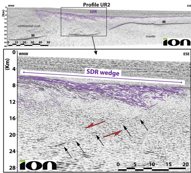
Fig. 5. Profile UR2 and close-up on a SDR wedge and associated Continentward Dipping Normal Fault. Data courtesy of ION Geophysical.
