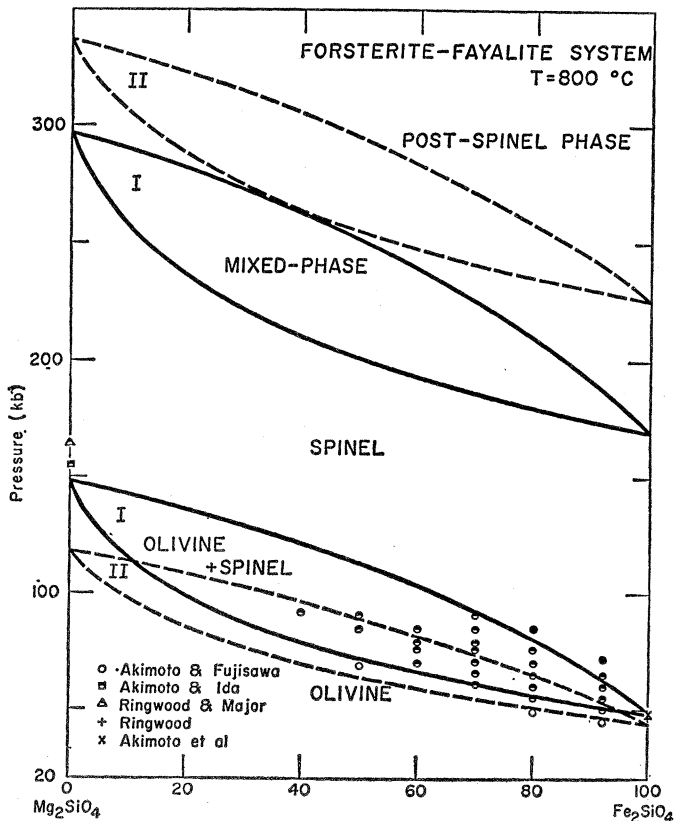
Fig. 3 (left). Estimated phase diagram for system Mg_2SiO_4-Fe_2SiO_4 using values for parameters from Tables 1 and 2. Calculations I and II are based on different pressure scales.
