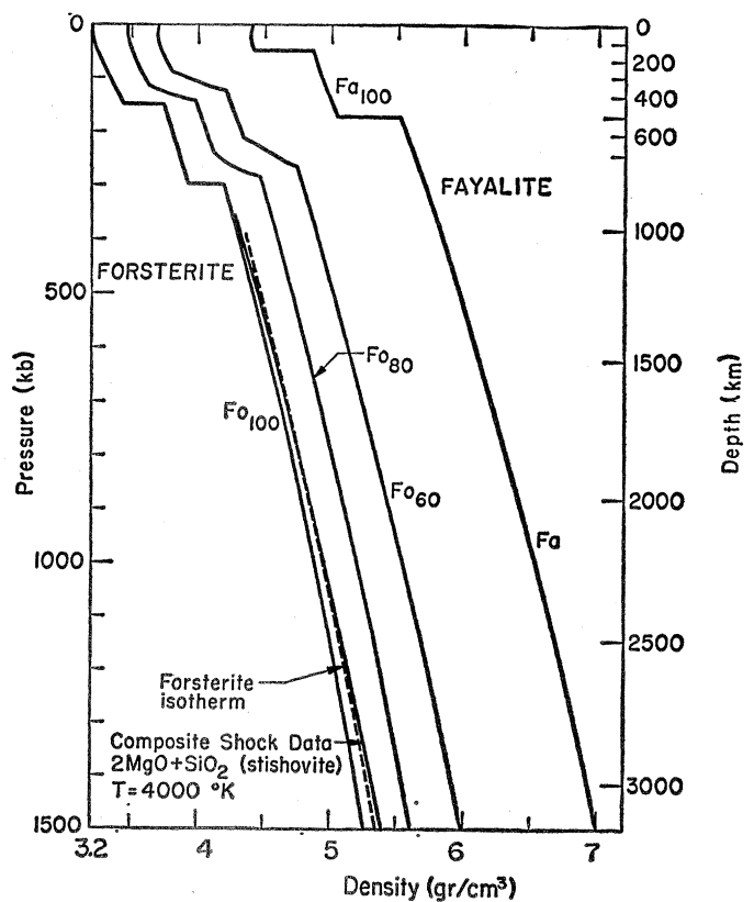
Fig. 4 (right). Density as a function of pressure and depth in the earth taking into account temperature, pressure, and solid-solid phase changes for olivine of four different compositions (22). Locations and details of transition regions computed at 800^\circ C .
