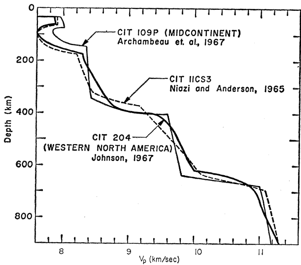
Fig. 1 (left). Compressional velocity versus depth in the upper mantle.
