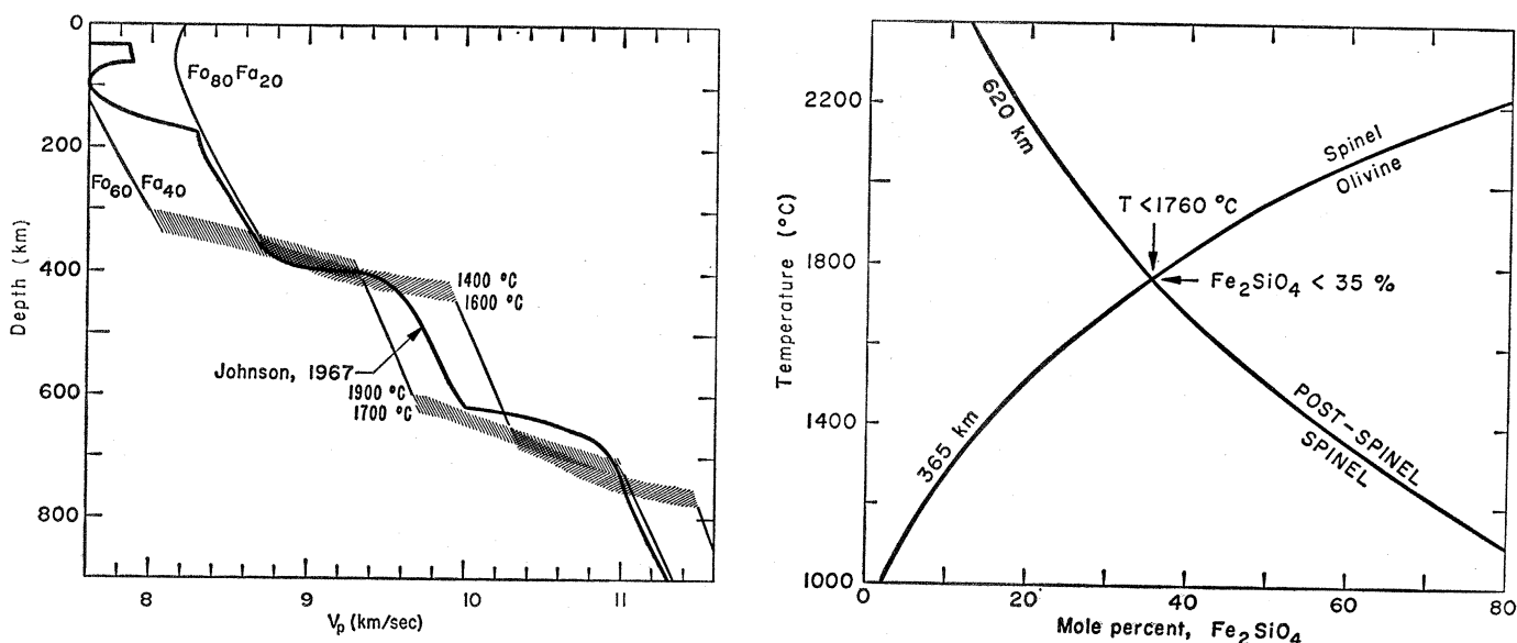
Fig. 5 (left). Compressional velocity, V_P , as a function of depth for Fo_{80}Fa_{20} and Fo_{60}Fa_{40} compared with seismic velocity structure of Johnson (4). Fig. 6 (right). Temperature and compositions in the mantle that are consistent with locations of seismic discontinuities at depths of 365 and 620 km.
