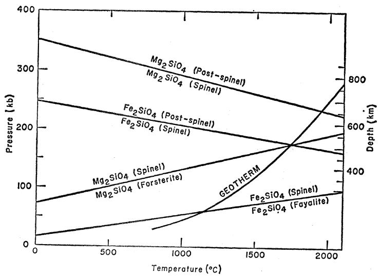
Fig. 2 (right). Equilibrium lines for olivine-spinel and spinel-oxides transformations in Mg_2SiO_4 and Fe_2SiO_4 .
