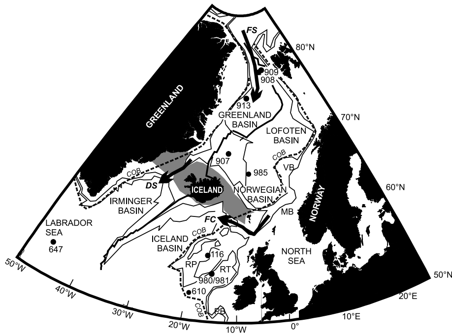
Fig. 1. Simplified map of NE Atlantic region showing: extent of NW European Atlantic continental margin (50°–70°N) covered in this study; the anomalously shallow Greenland–Scotland Ridge (grey); active mid-ocean spreading ridges; deep-water pathways (arrows); DSDP/ODP sites (solid black circles) referred to in the text; and the 1000 m and 2000 m bathymetric contours. RT, Rockall Trough; RP, Rockall Plateau; PB, Porcupine Basin; MB, Møre Basin; VB, Vøring Basin; FC, Faroe Conduit; DS, Denmark Strait; FS, Fram Strait; COB, Continent–Ocean boundary. The Møre and Vøring basins are presently buried beneath the Norwegian Shelf. In terms of the deep-water pathways, the Fram Strait represents the Northern Gateway whilst the Greenland–Scotland Ridge is the Southern Gateway.
