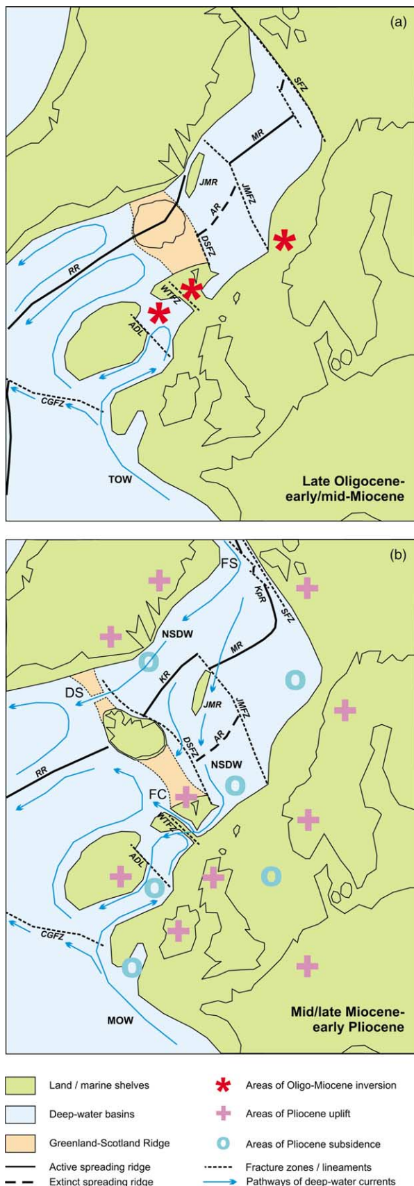
Fig. 11. Schematic reconstructions of NE Atlantic region for (a) late Oligocene–early/mid-Miocene, and (b) mid/late Miocene–early Pliocene intervals (see text for details). Plate tectonic framework based on Ziegler (1988). Abbreviations as in Figures 1 & 2 except: NSDW, Norwegian Sea Deep Water; TOW, Tethyan Outflow Water; MOW, Mediterranean Outflow Water; RR, Reykjanes Ridge; KR, Kolbeinsey Ridge; AR, Aegir Ridge; MR, Mohs Ridge; KpR, Knipovich Ridge; SFZ, Senja Fracture Zone; JMR, Jan Mayen Ridge.
