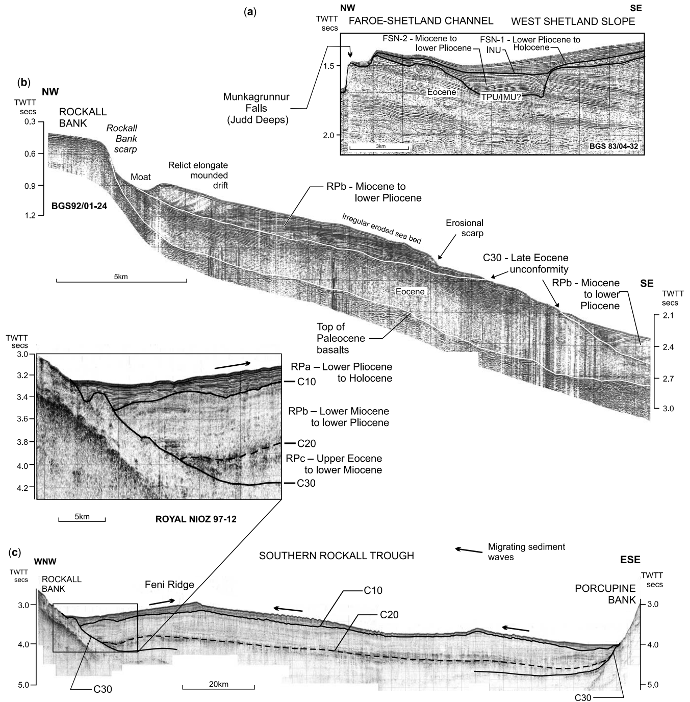
Fig. 7. (a) BGS airgun profile 83/04-32 showing the irregular nature of the TPU. Part of the surface is buried beneath an FSN-2 infilling drift and the lower part of the Rona Wedge slope apron (FSN-1); part remains open – the Munkagrannur Falls (Judd Deeps). This surface is locally composite with the IMU. (b) BGS airgun profile 92/01-24 across the western flank of the central Rockall Trough showing erosional sea bed, the relict middle-Miocene – lower Pliocene upslope prograding sediment drift, and locally exposed Eocene strata. (c) Royal NIOZ profile 97-12 across the southern Rockall Trough, between Rockall and Porcupine banks, highlighting the Feni Ridge sediment drift, a smaller subsidiary drift adjacent to Porcupine Bank, sediment waves at sea bed, and wide erosional moats adjacent to the banks. Inset shows details of the basin-margin and moated areas, particularly the erosional nature of C10.
