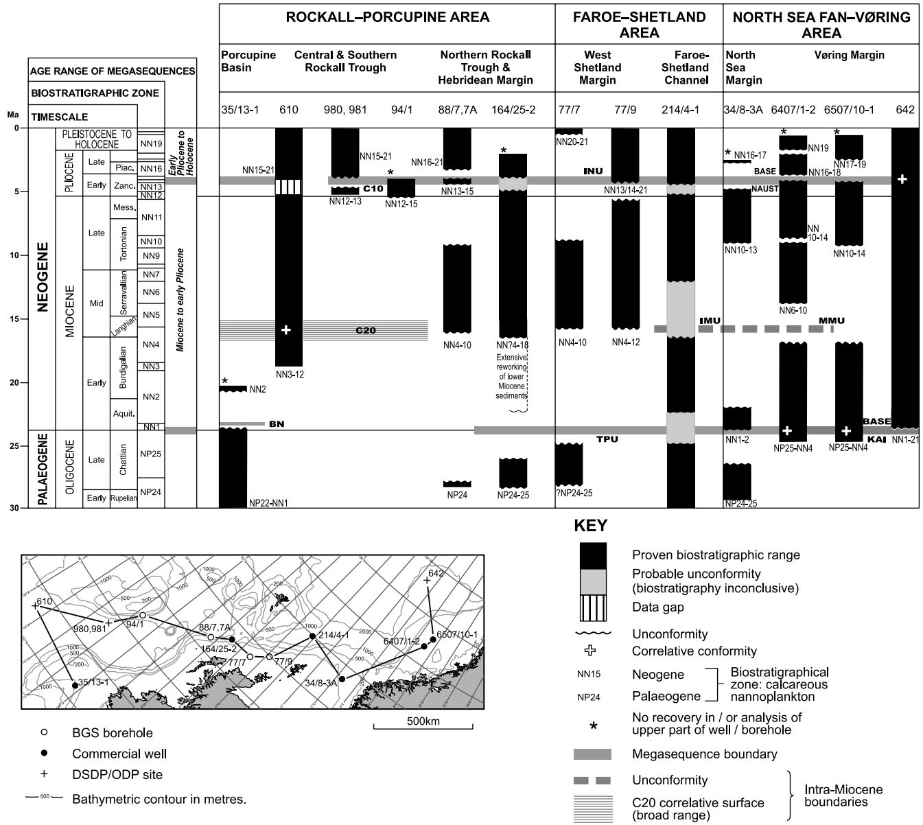
Fig. 5. Stratigraphical-range chart of key boreholes and wells used in the calibration and correlation of key Neogene reflectors along the NW European Atlantic margin. Timescale is from Berggren et al. (1995a). BN, Base Neogene in Porcupine Basin; TPU, Top Palaeogene Unconformity; IMU, Intra-Miocene Unconformity; MMU, Mid-Miocene Unconformity; INU, Intra-Neogene Unconformity. See text for details.
