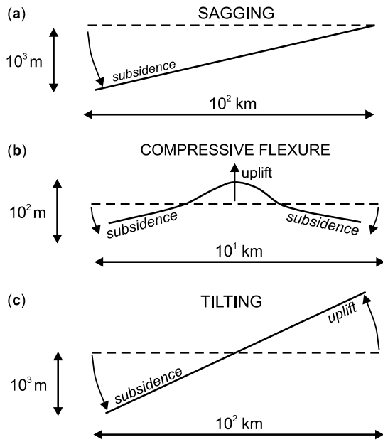
Fig. 9. Types of differential vertical movements recognised on the NW European margin in the mid- to late Cenozoic: (a) sagging (mid-Cenozoic); (b) compressive flexure (early–mid-Miocene); (c) tilting (early Pliocene).
