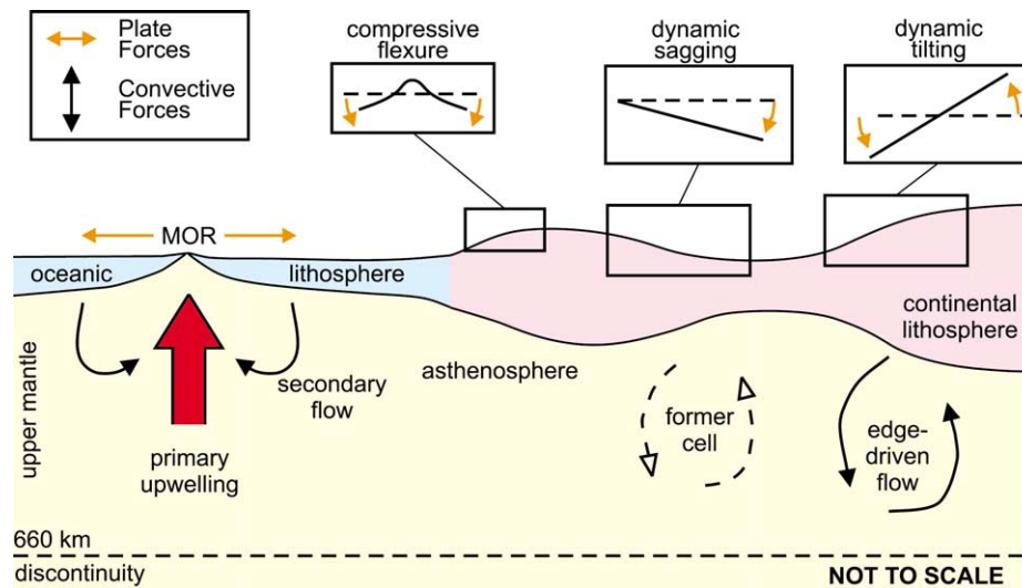
Fig. 12. Conceptual diagram (not to scale) showing the interaction of forces within the upper mantle and lithosphere across a developing ocean basin, along with the differing structural and topographic responses hypothesized for the NW European continental margin in the late Palaeogene and Neogene. Upper mantle convective cells may arise due to temperature inhomogeneities at the base of the lithosphere, such as across the ocean–continent boundary or a deep-water basin; the inferred dynamic topographic response to edge-driven flow corresponds to the late Eocene–early Oligocene sagging and early Pliocene tilting observed along the margin. Variations in horizontal forces within the European plate resulted in compressive flexure throughout the Cenozoic, culminating in the early to mid-Miocene development of inversion anticlines and basin margin unconformities. MOR, Mid-Ocean Ridge.
