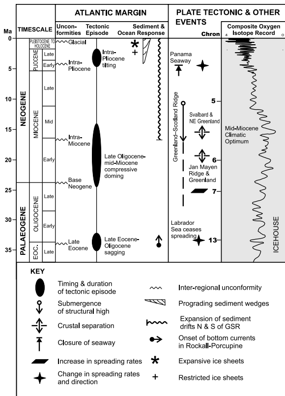
Fig. 10. Neogene tectonostratigraphic framework for the NW European Atlantic margin (see text for details). Timescale from Berggren et al. (1995a).
