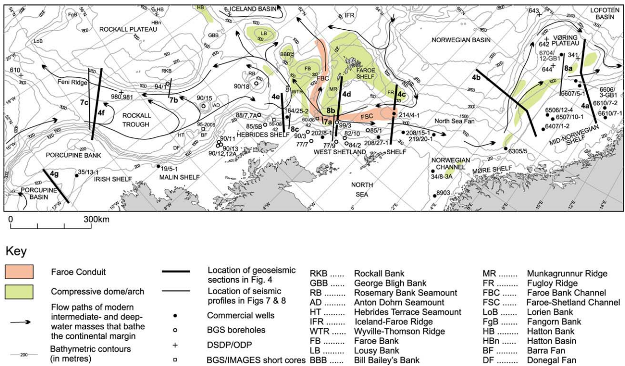
Fig. 3. Detailed map of study area showing locations of sample sites, geoseismic sections and seismic profiles referred to in text and other figures.
