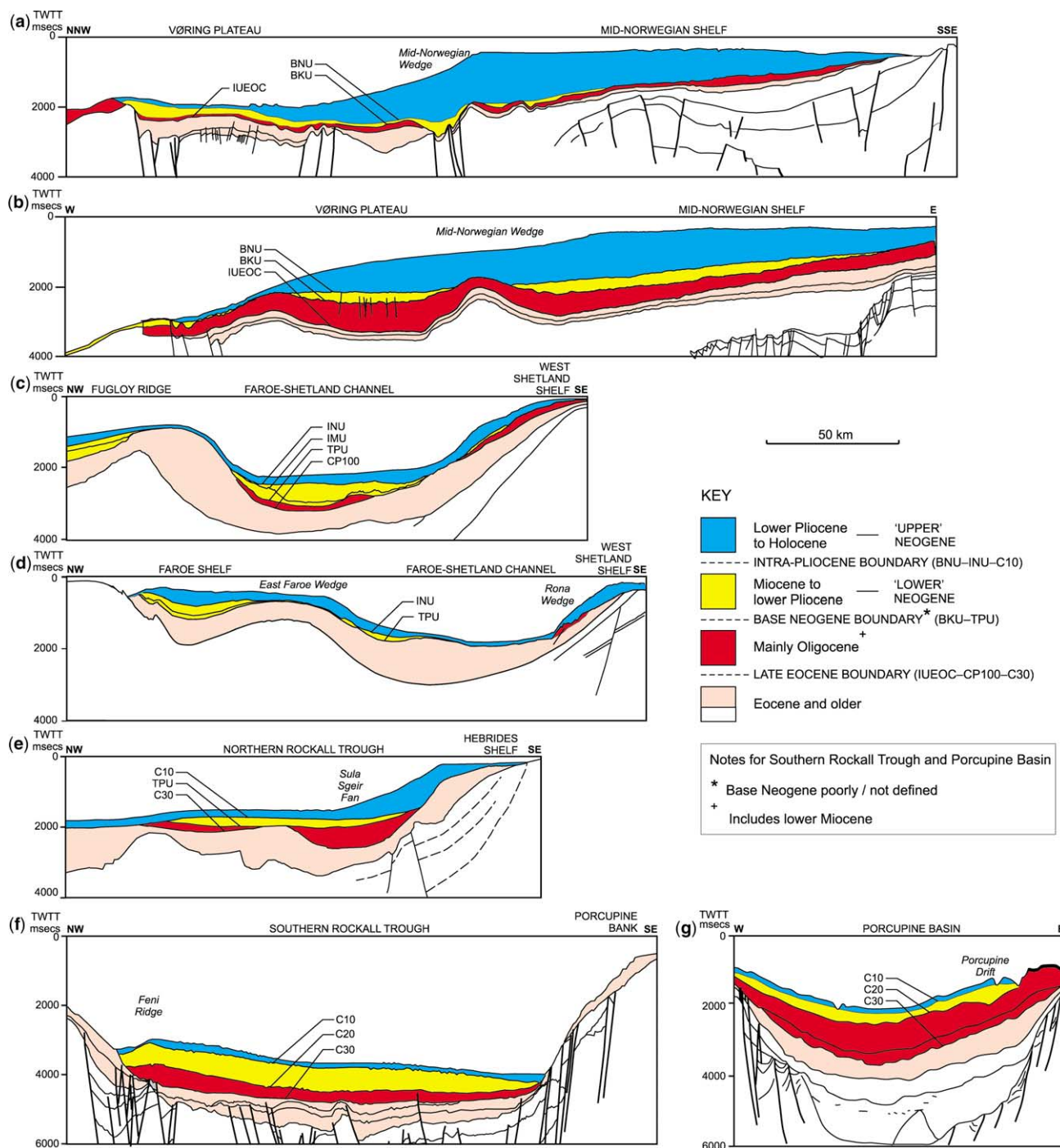
Fig. 4. Interpreted geoseismic sections along the NW European Atlantic margin, focusing on the middle to upper Cenozoic stratigraphy. Sections (a) and (b) simplified from profiles D–D' and J–J' of Blystad et al. (1995); section (c) based on profile OF94-55a (Faroe margin) and BGS profile 84/05-10 (West Shetland margin); section (d) based on profile OF94-25a (Faroe margin) and BGS profile 83/04-29 (West Shetland margin); section (e) based on profile DG95-10; section (f) based on profile GSR96-0116; section (g) based on profile MS-81-25 and simplified from McDonnell & Shannon (2001). Location of sections shown in Figure 3. Abbreviations: BNU, Base Naust Unconformity; INU, Intra-Neogene Unconformity; BKU, Base Kai Unconformity; TPU, Top Palaeogene Unconformity; IUEOC, Intra-Upper Eocene Unconformity; IMU, Intra-Miocene Unconformity. TWTT, two-way travel time.
