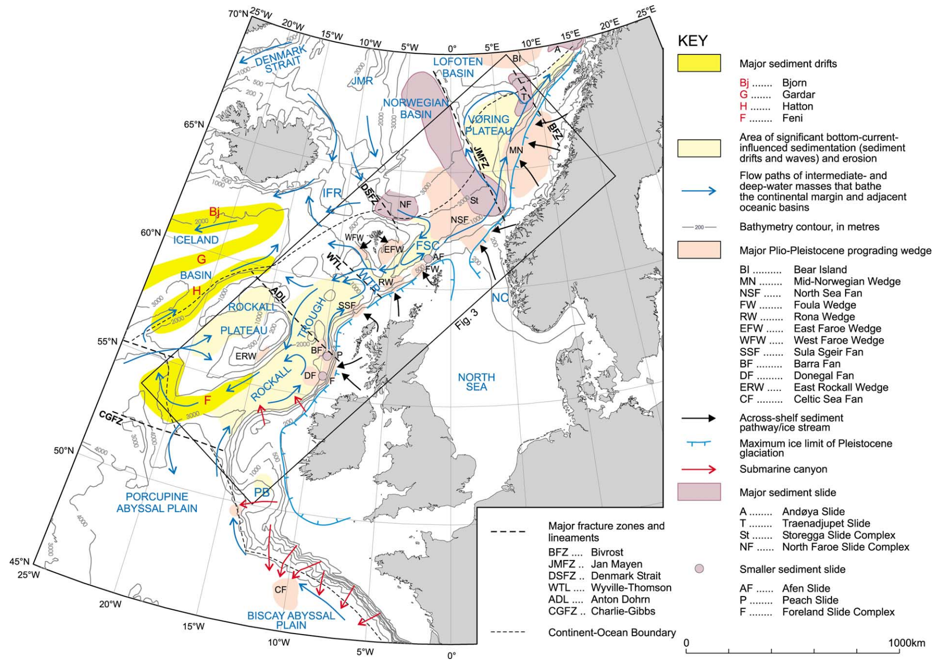
Fig. 2. Bathymetric setting of the NW European Atlantic margin showing location of study area (boxed), main tectonic elements, oceanographic circulation pattern, and summary of large-scale sedimentary processes that have contributed to the shaping of the ocean margin during the Neogene. Study area is expanded in Figure 3. NC, Norwegian Channel; FSC, Faroe–Shetland Channel; IFR, Iceland–Faroe Ridge; WTR, Wyville–Thomson Ridge; PB, Porcupine Basin; JMR, Jan Mayen Ridge.
