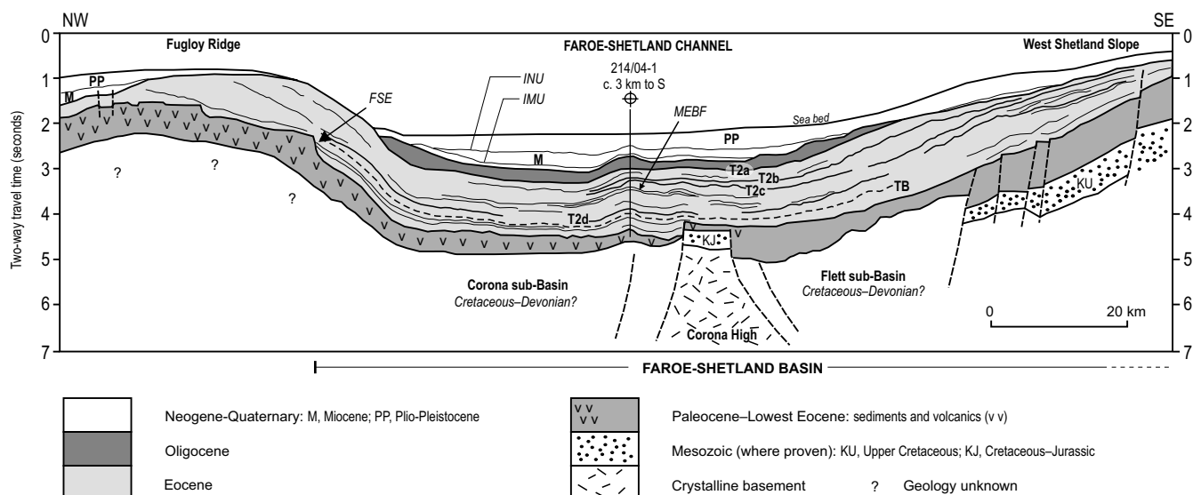
FIG. 2. Geoseismic section showing the general structural disposition of the Eocene succession in the Faroe-Shetland region, including the key Eocene (Stronsay Group) seismic boundaries, T2a–T2d. FSE, Faroe-Shetland Escarpment; IMU, intra-Miocene unconformity; INU, Intra-Neogene unconformity; MEBF, Middle Eocene basin-floor sandstones; TB, Top Balder Fm. Section is located in Figure 1.
