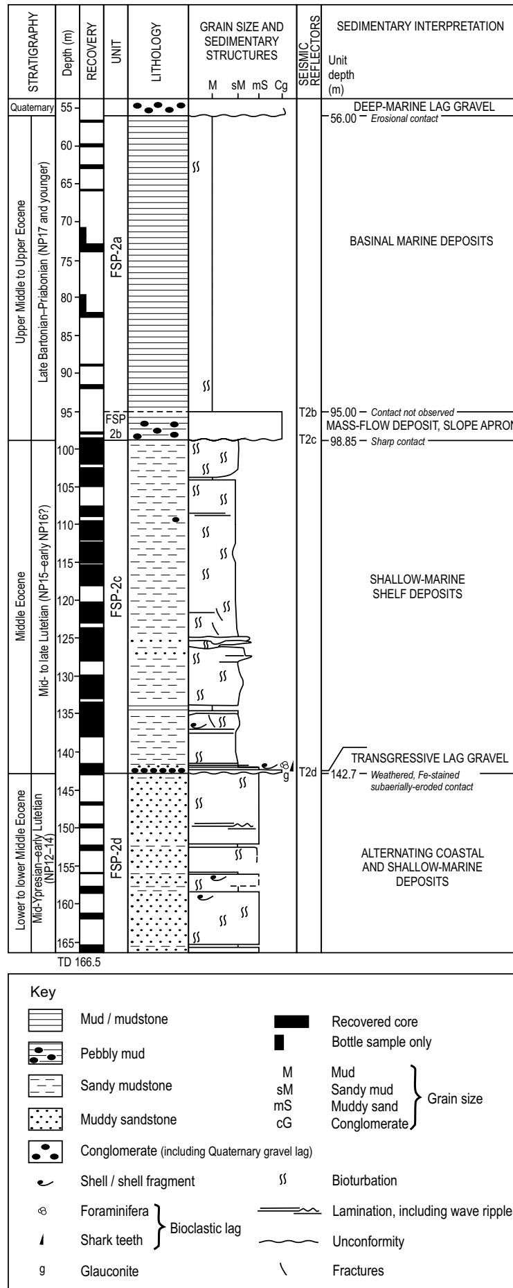
FIG. 4. Graphic log of Eocene succession in BGS borehole 99/3 (see text for details). Depth in metres, below sea bed.
