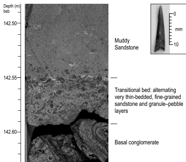
FIG. 6. Basal conglomerate of unit FSP-2c passing transitionally upwards into muddy sandstone. Inset shows shark tooth recovered from the conglomerate. bsb, below sea bed.
