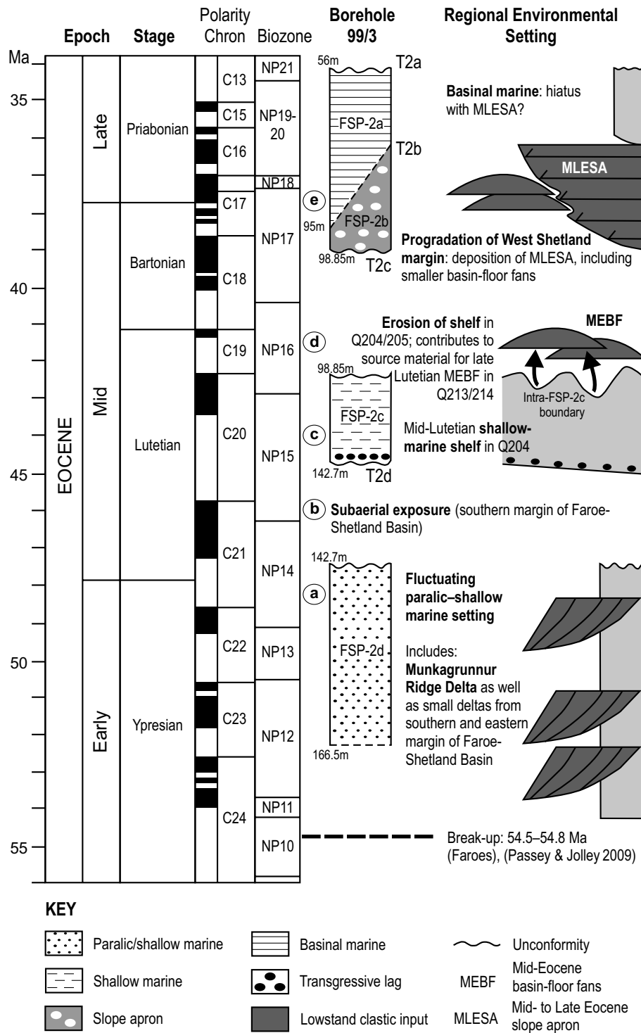
FIG. 7. Stratigraphical-range and palaeoenvironmental setting of Eocene rocks in BGS borehole 99/3 (see text for details). Circled letters (a) to (e) relate to position of timeslice intervals illustrated in Figure 8. Core depths are cross-referenced to graphic log in Figure 4. Timescale from Gradstein et al. (2012). Q, Quadrant.
