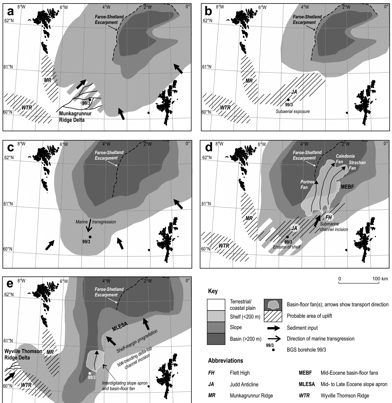
FIG. 8. Series of schematic palaeogeographical maps showing the inferred spatial and temporal development of the Faroe-Shetland Basin during Eocene times: (a) late Ypresian–earliest Lutetian; (b) early/mid-Lutetian; (c) mid-Lutetian; (d) late Lutetian; (e) late Bartonian–Priabonian. Palaeogeographical information derived from: Waagstein & Heilmann-Clausen (1995), Andersen et al. (2000), Brooks et al. (2001), Robinson (2004), Robinson et al. (2004), Smallwood (2004); Ritchie et al. (2008), Ólavsdóttir et al. (2010), Tuitt et al. (2010), Stoker & Varming (2011) and unpublished BGS data (see text for details).
