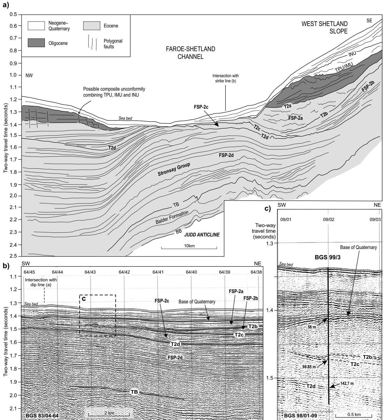
FIG. 3. Geological setting of BGS borehole 99/3. (a) Line drawing showing seismic stratigraphy and structural disposition of Eocene (syn-break-up Balder Formation and post-break-up Stronsay Group) in the area of the borehole (modified after Stoker & Varming 2011). (b) BGS airgun profile 83/04-64 along axis of Faroe-Shetland Channel showing downlap of reflector T2b on to T2c, and concomitant pinchout of unit FSP-2b towards borehole site. (c) BGS sparker profile 98/01-9 showing high-resolution seismic stratigraphy at borehole site calibrated to depth in metres, below sea bed, based on a two-way time of 1500 \text{ m s}^{-1} for the unconsolidated section above 98.85 m, and 2000 \text{ m s}^{-1} for the lithified section below this depth. Location of profiles is shown in Figure 1. BB, Base Balder Fm; TB, Top Balder Fm; IMU, intra-Miocene unconformity; INU, intra-Neogene unconformity; TPU, Top Palaeogene unconformity.
