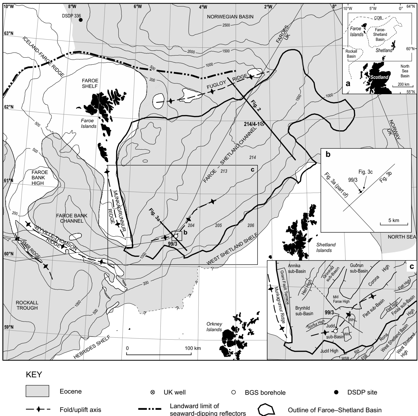
FIG. 1. Map showing location and present-day physiography of study area, general distribution of the Eocene succession, BGS borehole 99/3, DSDP site 336 and well 214/4-1, and UK Quadrants referred to in text; also, position of profiles shown in Figures 2 and 3. Inset (a) shows regional setting of Farø–Shetland Basin. COB, continent–ocean boundary. Inset (b) shows detailed layout of profiles in Figure 3 relative to borehole 99/3. Inset (c) shows early post-break-up structural setting of the southwestern end of the Farø–Shetland Basin (from Ritchie et al. 2011). COB, continent–ocean boundary; ESB, East Solan Basin; RH, Rona High; WH, Westray High; WSB, West Solan Basin; (other) DSDP, Deep Sea Drilling Project. Bathymetric contours in metres.
