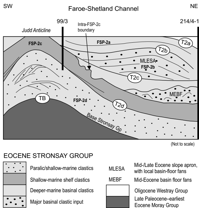
FIG. 5. Schematic section along the axis of the Faroe–Shetland Channel showing the general relationship of the Eocene seismic-stratigraphical units (FSP-2a–FSP-2d) and key reflectors (T2a–T2d; intra-FSP-2c) correlated between BGS borehole 99/3 (Quadrant 204) and well 214/4-1 (Quadrant 214). TB, Top Balder Formation.
