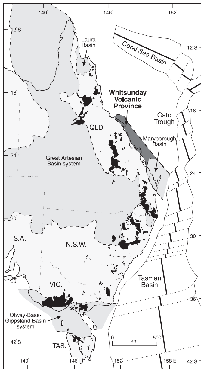
Figure 4. Location of the silicic-dominated Whitsunday volcanic province (132–95 Ma) and Early Cretaceous sedimentary basins of eastern Australia that contain >1.4 × 10 6 km 3 of coeval large igneous province-derived volcanogenic sediment (Bryan et al., 1997). Large igneous province magmatism was followed by: (1) kilometer-scale uplift of eastern margin of Australia beginning ca. 100–95 Ma (e.g., O’Sullivan et al., 1995, 1999); (2) seafloor spreading in Tasman Basin–Cato Trough–Coral Sea Basin occurring between 84 and 56 Ma (e.g., Veever et al., 1991); and (3) intraplate alkaline volcanism (80–0 Ma, shown in black) that was partly synchronous with seafloor spreading, and that defines a broken belt 4400 km long along the highlands of eastern Australia. Intraplate alkaline volcanism occurred within 500 km of coastline, and has an extrusive volume of >20 000 km 3 (Johnson, 1989). QLD, Queensland; N.S.W., New South Wales; VIC., Victoria; TAS., Tasmania; S.A., South Australia.
