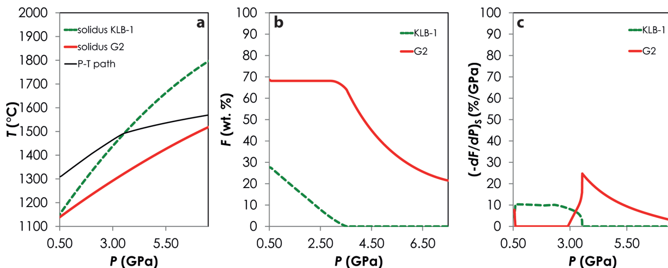
Figure S-1 Results of the Melt-PX calculations for the G2-configuration at a potential temperature of 1480 °C. (a) Pressure-temperature path for the column of mantle undergoing isentropic decompression (black line). The solid red and the dashed green lines are the solidi of G2 and KLB-1, respectively. (b-c) Extent of the melting (b) and melt productivity (c) of G2 (solid red line) and KLB-1 (dashed green line) along the adiabatic path.
